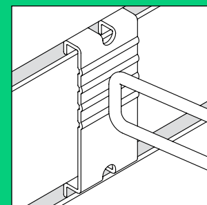
F4 - Fastback 4® Slatwall Back
