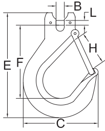
Stamped with BM identification code, size, grade and traceability code. Meet ASTM-952 standard.
