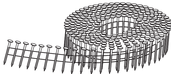
Wire Collation
