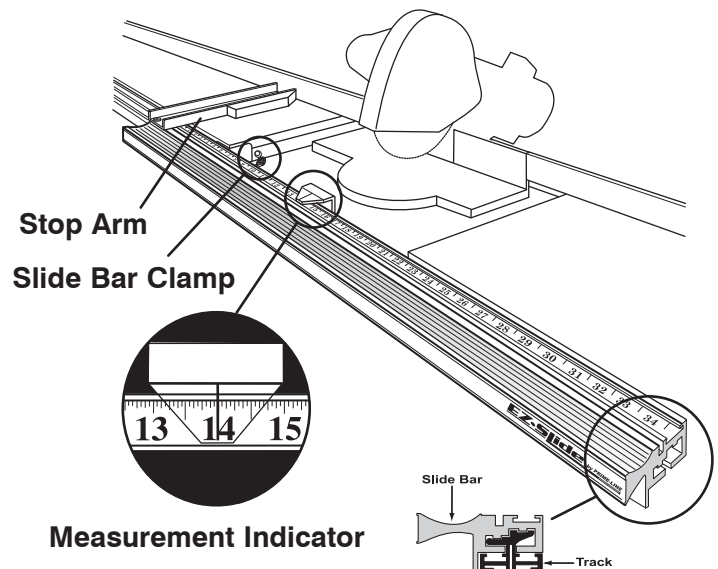
P-7926 (LH-Stop) Shown
