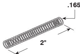
Slide Bolt Spring
