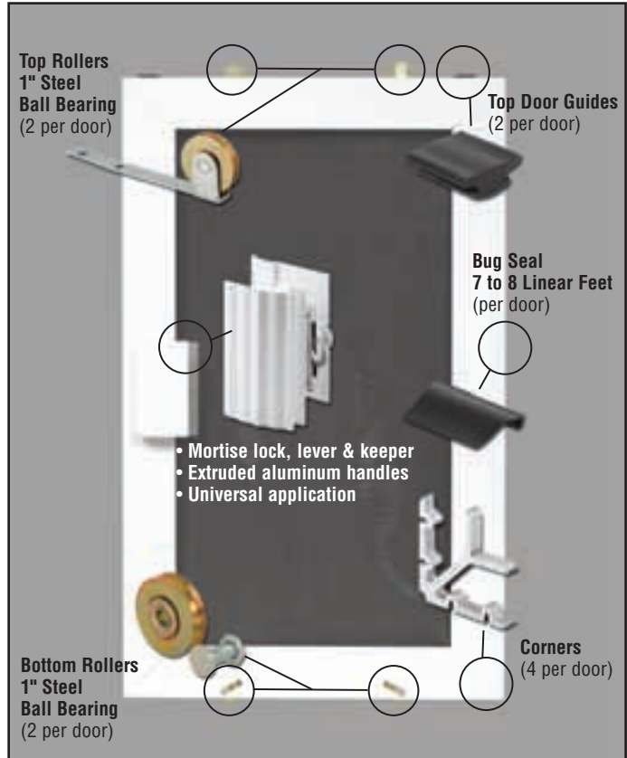
Ultimate II (2-1/2")
