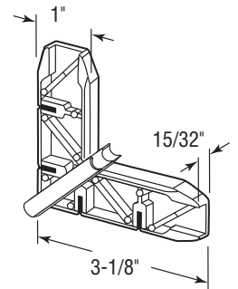
Plastic Outside Miter
