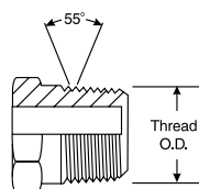
BSPT Male (MBSPT)
