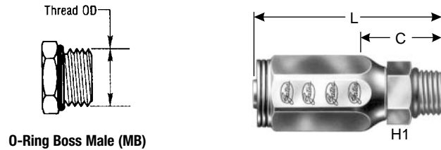
O-Ring Boss Male (MB)
