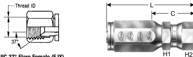
JIC 37° Flare Female (FJX)
