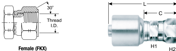
Female (FKX)
