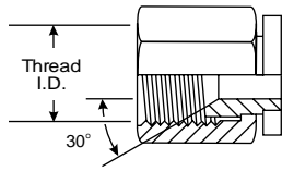
Japanese 30° Flare Female
