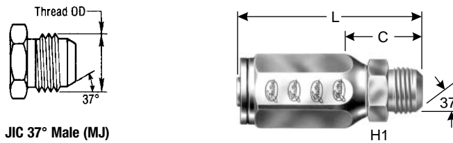
JIC 37° Male (MJ)
