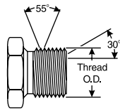
BSPP Male
