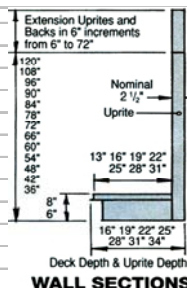
WALL SECTIONS
