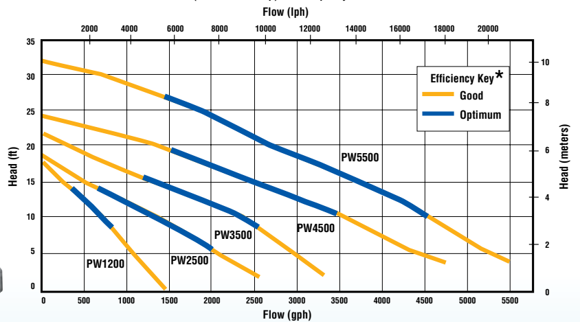
(PW-Series Pump) Head-Capacity Curves
