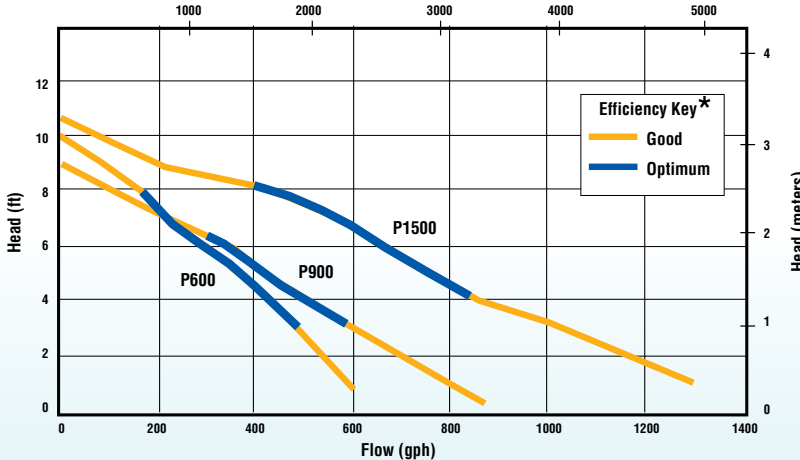
(P-Series Pump) Head-Capacity Curves Flow (lph)
