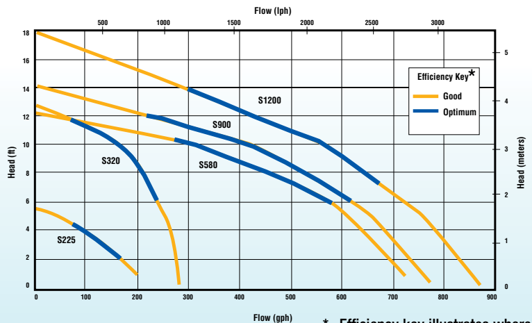
(S-Series Pump) Head-Capacity Curves
