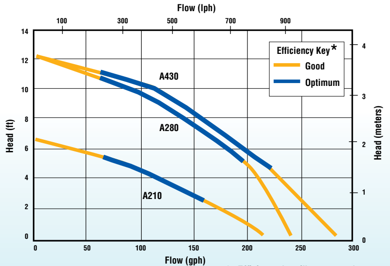
(A-Series) Pump Head-Capacity Curves
