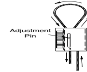
Step 5 To adjust, remove tension and pull wire rope slightly to disengage teeth, slide adjustment pin in direction shown by arrow to release wire rope
