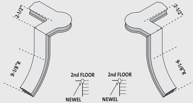
SP107 1 Riser 1/4 Turn With Cap - Left SP107-40C - PC
