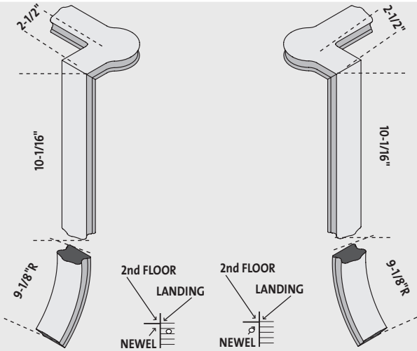
SP109 2 Riser 1/4 Turn With Cap - Left SP109-40C - PC
