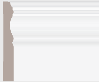
00706 9/16" x 4-1/8" 00706-30096C - 8' 00706-30192C - 16'
