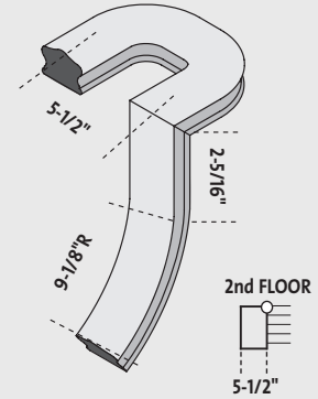
SP112 1 Riser Floor Return - Left SP112-40C - PC
