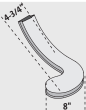
SP093 1/2 Volute Left SP093-40C - PC
