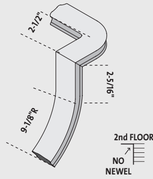
SP103 1 Riser 1/4 Turn No Cap - Left SP103-40C - PC
