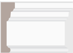
95010 Architrave 1-3/16" x 4-3/16" 95010-90042CB1 - 42" PFJ Pine
