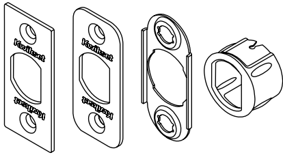
6-Way Deadlatch Service Kit
