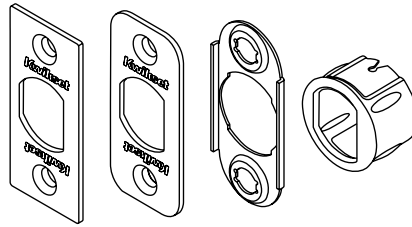
6-Way Plain Latch Service Kit
