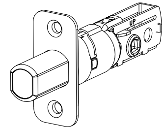
RC Adjustable Deadbolt Latch
