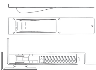
7802 Double-Acting w/ Jamb Bracket
