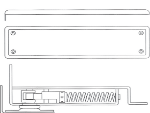
7812 Double-Acting Heavy Duty w/ Jamb Bracket
