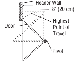
One-piece door without track: pivot hardware
