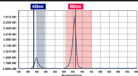
SPECTRAL POWER DISTRIBUTION CURVE
