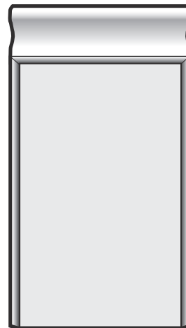
PLINTH BLOCK - COLONIAL Primed LDF 3/4" x 3-3/8" x 6" 06205-96C – $1.990/PC For Corner Block 06909-96C
