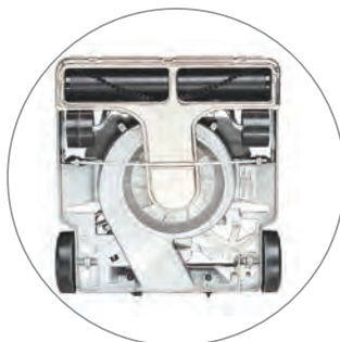
Clear quick release fan chamber makes service and clean-up easy
