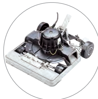
Virtually unbreakable all metal chassis for extended life
