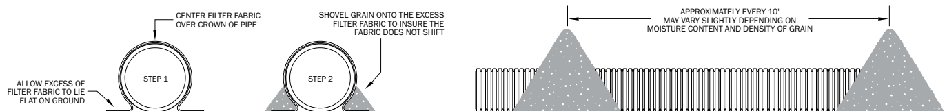
GRAIN-AIRE PIPE
